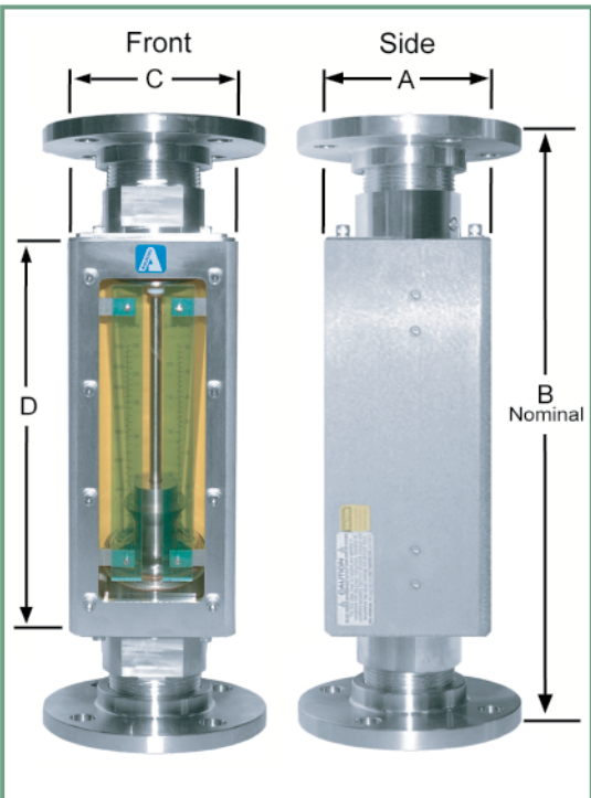
DIMENSIONS FOR FLANGED M STYLE METERS
